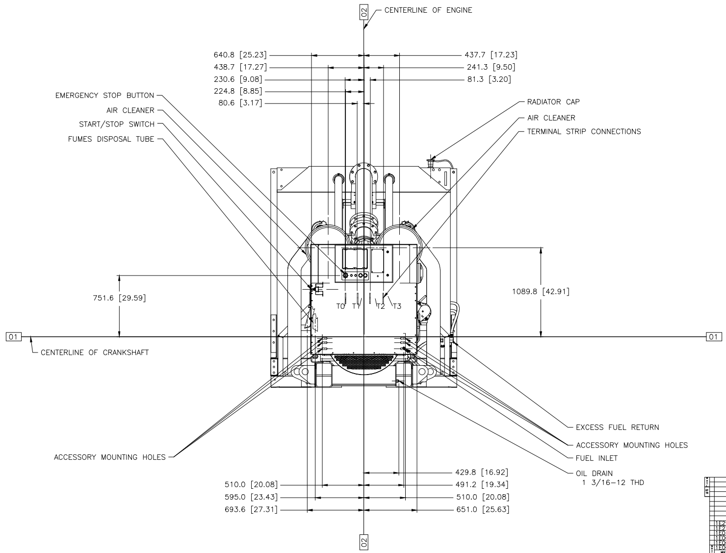
CAT 3512C LV 60HZ GENSET DWG# 521-8327 CHG 01 METRIC [INCH] REAR VIEW LF-2923 CHG 03 SHOWN
