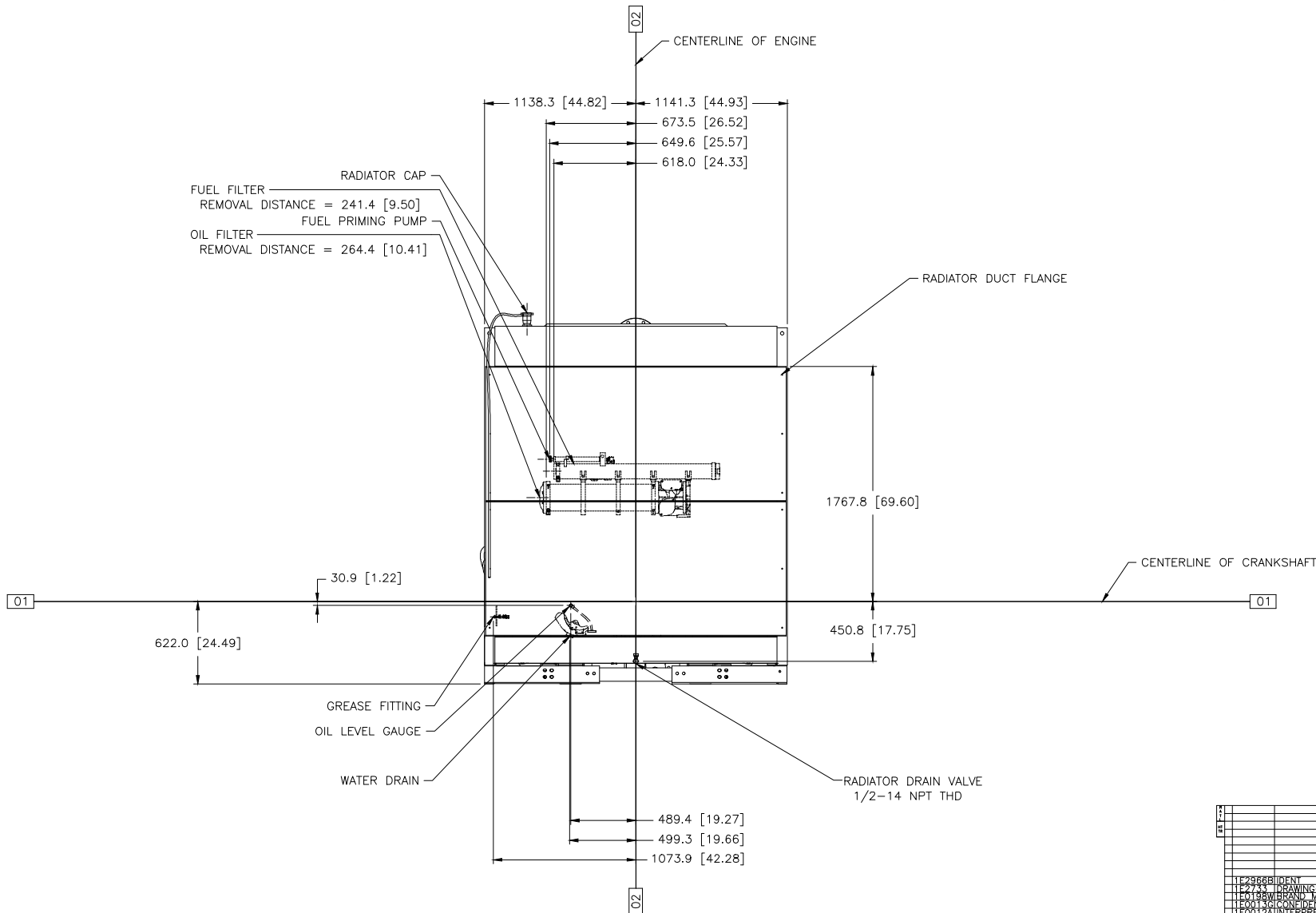
CAT 3512C-HD LV 60HZ 1750KW GENSET DWG# 521-8329 CHG 02 METRIC [INCH] FRONT VIEW LF-2925 CHG 03 SHOWN
