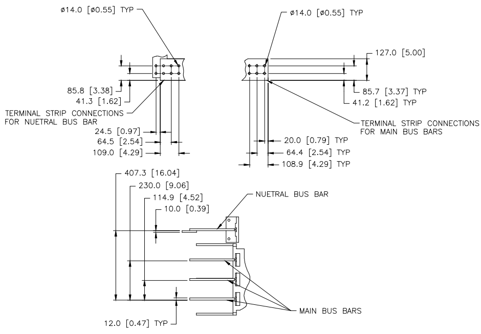
DETAIL OF TERMINAL STRIP CONNECTIONS SCALE 1=5
