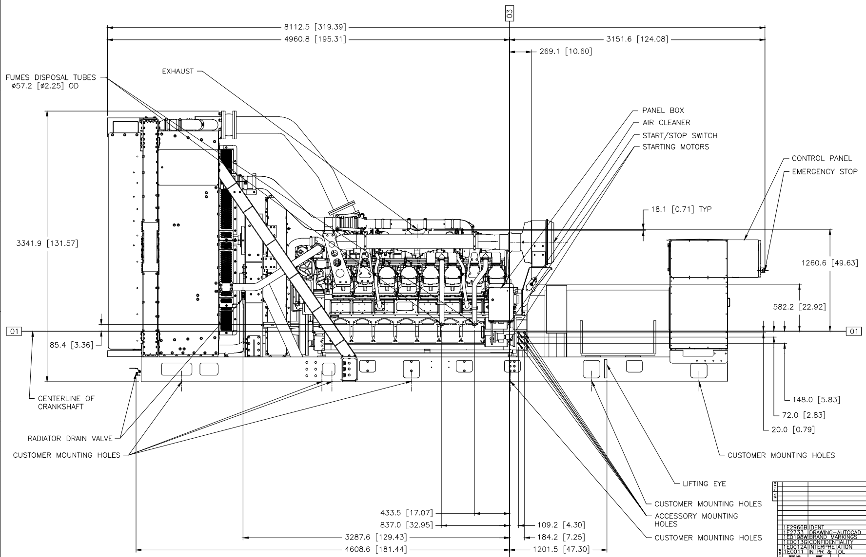
CAT 3516E 60HZ LV/MV PKG 2750KW DWG# 546-4171 CHG 01 METRIC [INCH] LEFT SIDE VIEW LF-3213 CHG 00 W/ATTACHMENTS SHOWN
