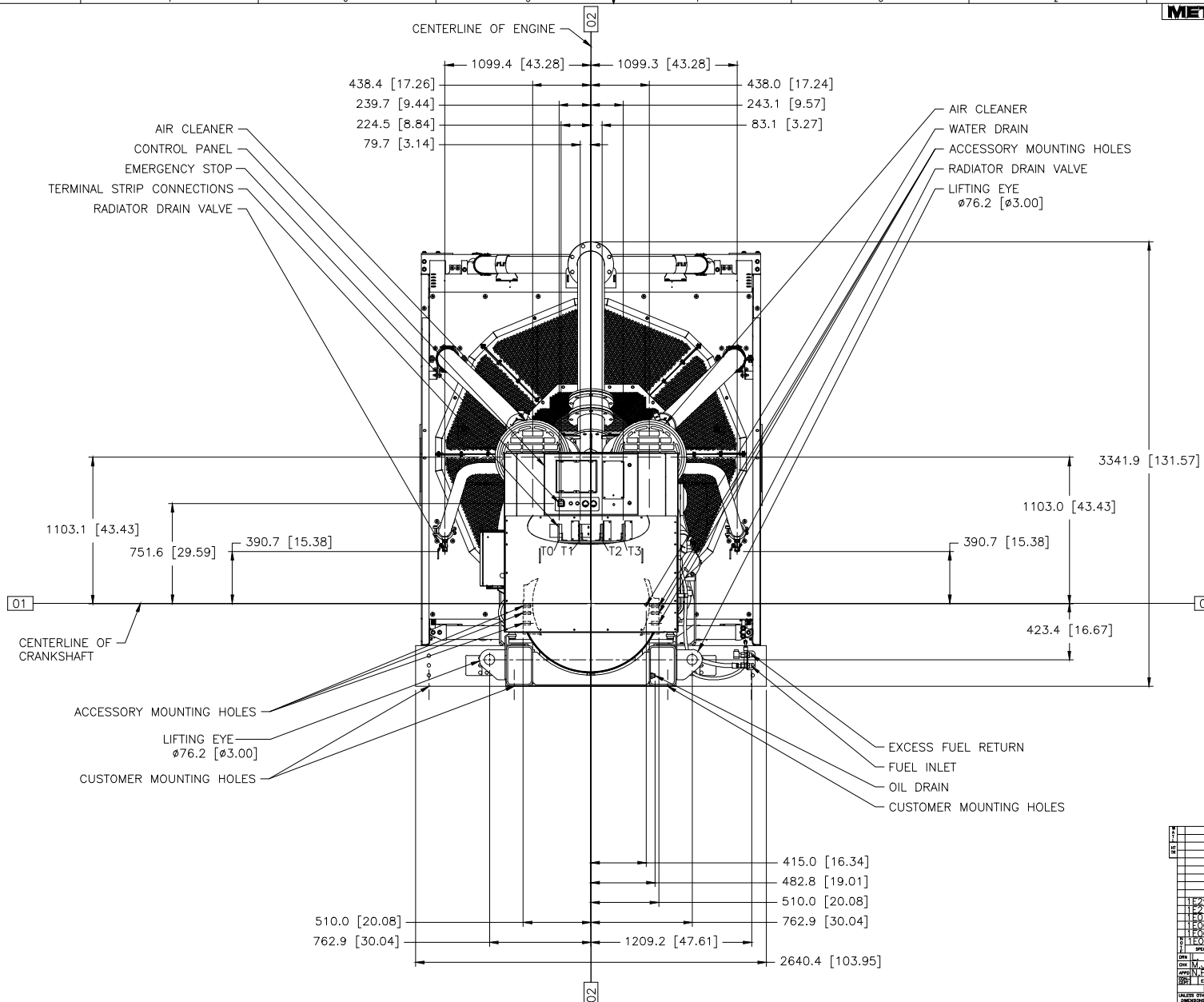
CAT 3516E 60HZ LV/MV PKG 2750KW DWG# 546-4171 CHG 01 METRIC [INCH] REAR VIEW LF-3213 CHG 00 W/ATTACHMENTS SHOWN
