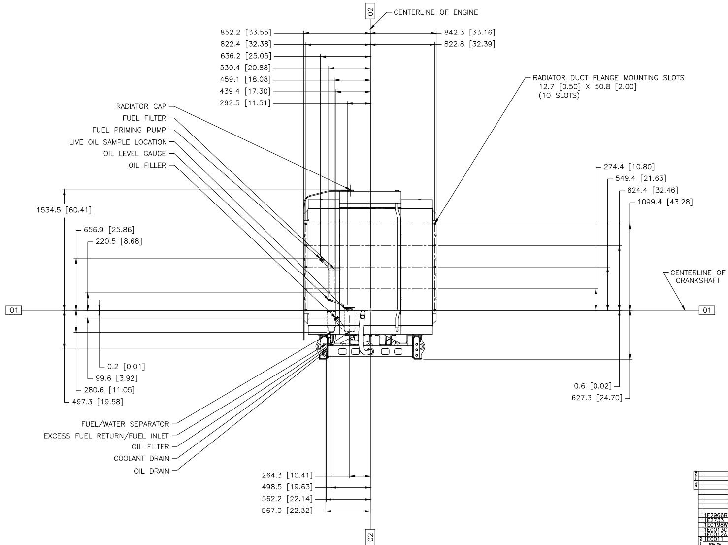
CAT C32 50/60HZ 1500RPM T2/LOW BSFC W/STD OIL PAN & RADIATOR DWG# 522-7044 CHG 02 METRIC [INCH] FRONT VIEW LF-3554 CHG 02 W/ MANDATORY ATTACHMENTS SHOWN
