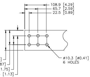
DETAIL OF TERMINAL STRIP CONNECTIONS 447-1538 CHG 01 SCALE 1=2
