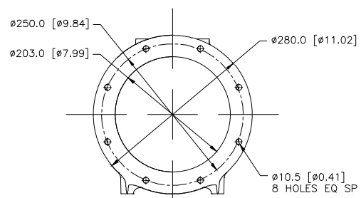
DETAIL OF EXHAUST SCALE 1=2
