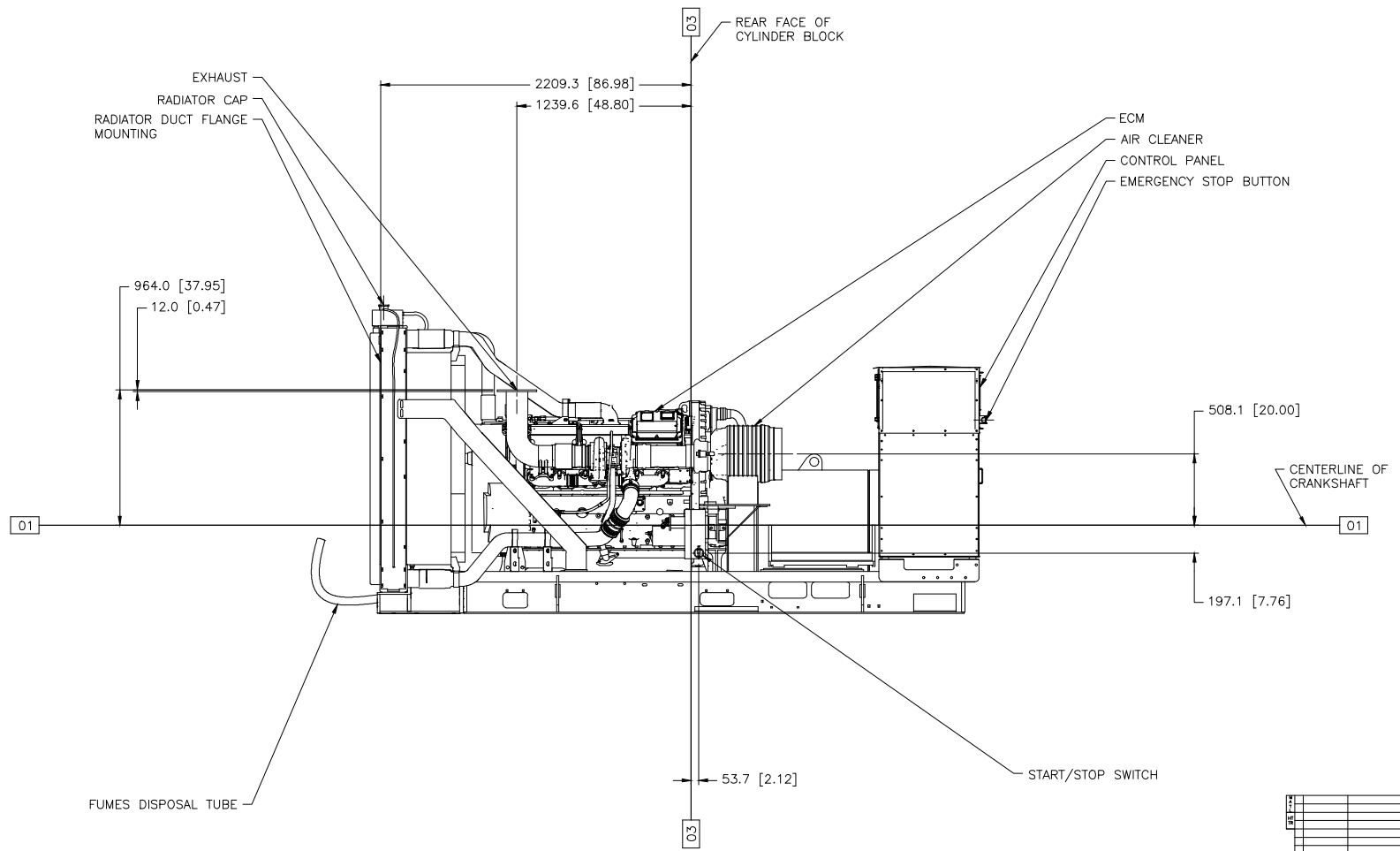
CAT C32 60HZ 1500RPM T2/LOW BSFC W/STD OIL PAN & RADIATOR DWG# 554-1977 CHG 02 METRIC [INCH] LEFT SIDE VIEW LF-3643 CHG 03 W/ MANDATORY ATTACHMENTS SHOWN
