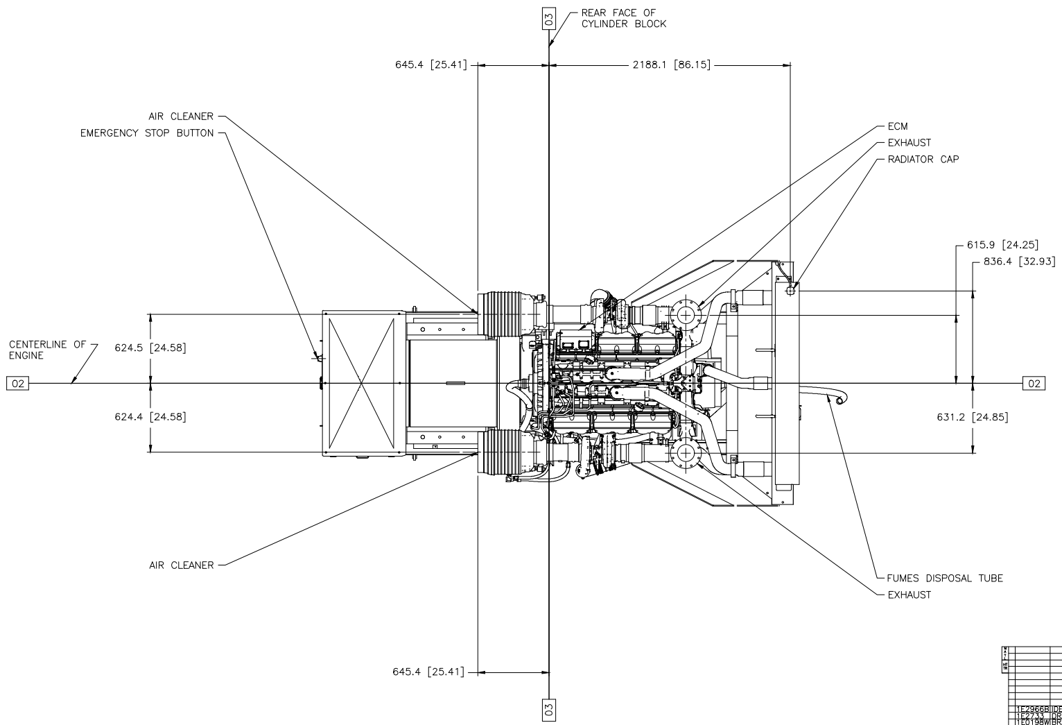
CAT C32 60HZ 1500RPM T2/LOW BSFC W/STD OIL PAN & RADIATOR DWG# 554-1977 CHG 02 METRIC [INCH] TOP VIEW LF-3643 CHG 03 W/ MANDATORY ATTACHMENTS SHOWN
