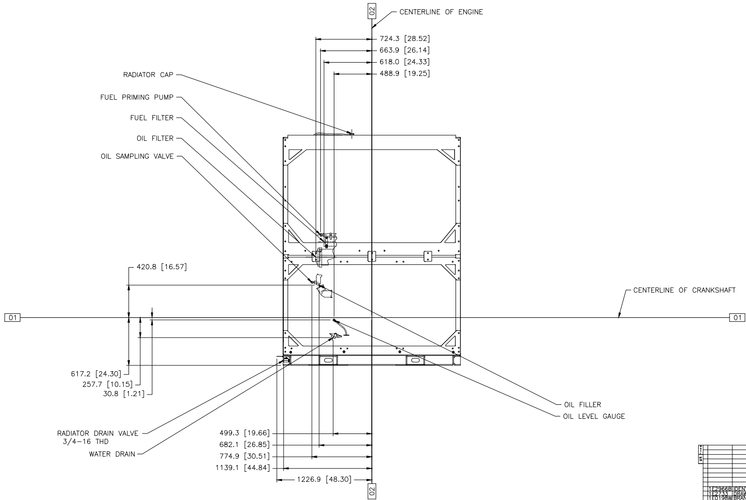
CAT 3516CHD 60HZ LV/MV PKG DWG# 590-8248 CHG 01 METRIC [INCH] FRONT VIEW LF-4462 CHG 00 W/ATTACHMENTS SHOWN
