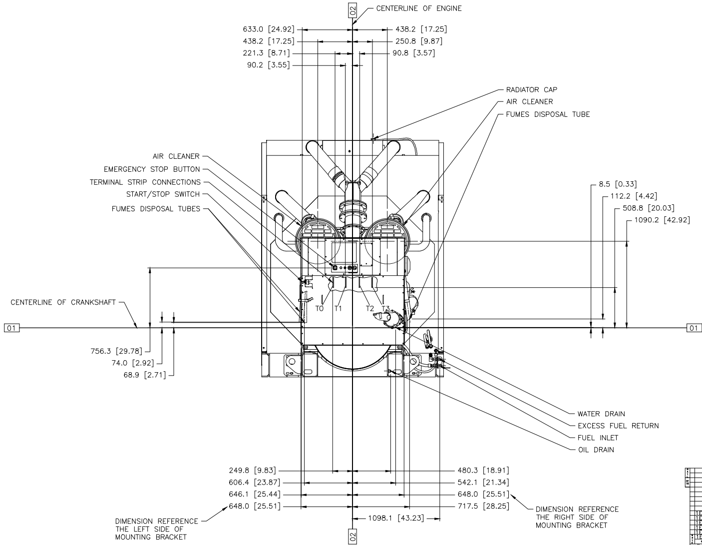
CAT 3516CHD 60HZ LV/MV PKG DWG# 590-8248 CHG 01 METRIC [INCH] REAR VIEW LF-4462 CHG 00 W/ATTACHMENTS SHOWN
