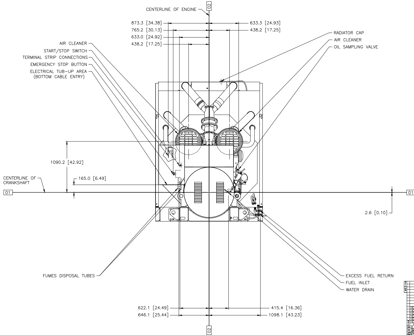
CAT 3516C 60HZ HV 1825/2000 KW DWG# 593-3168 CHG 01 METRIC [INCH] REAR VIEW LF-4453 CHG 00 W/ATTACHMENTS SHOWN
