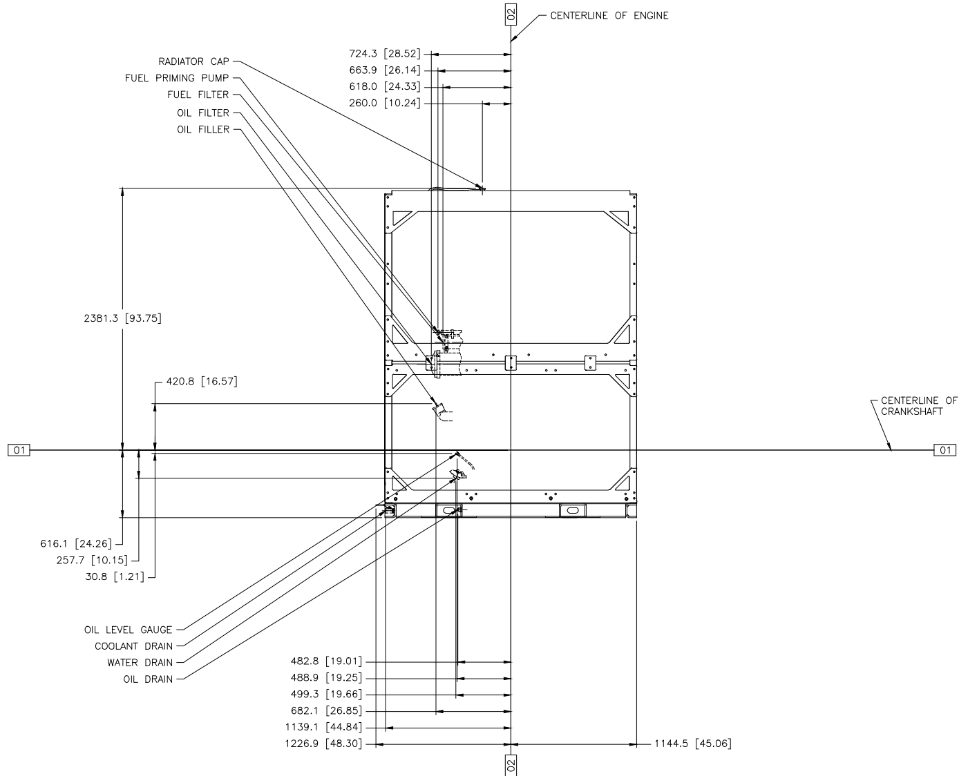
CAT 3516CHD 60HZ HV 2250/2500 KW DWG# 593-3169 CHG 01 METRIC [INCH] FRONT VIEW LF-4465 CHG 00 W/ATTACHMENTS SHOWN
