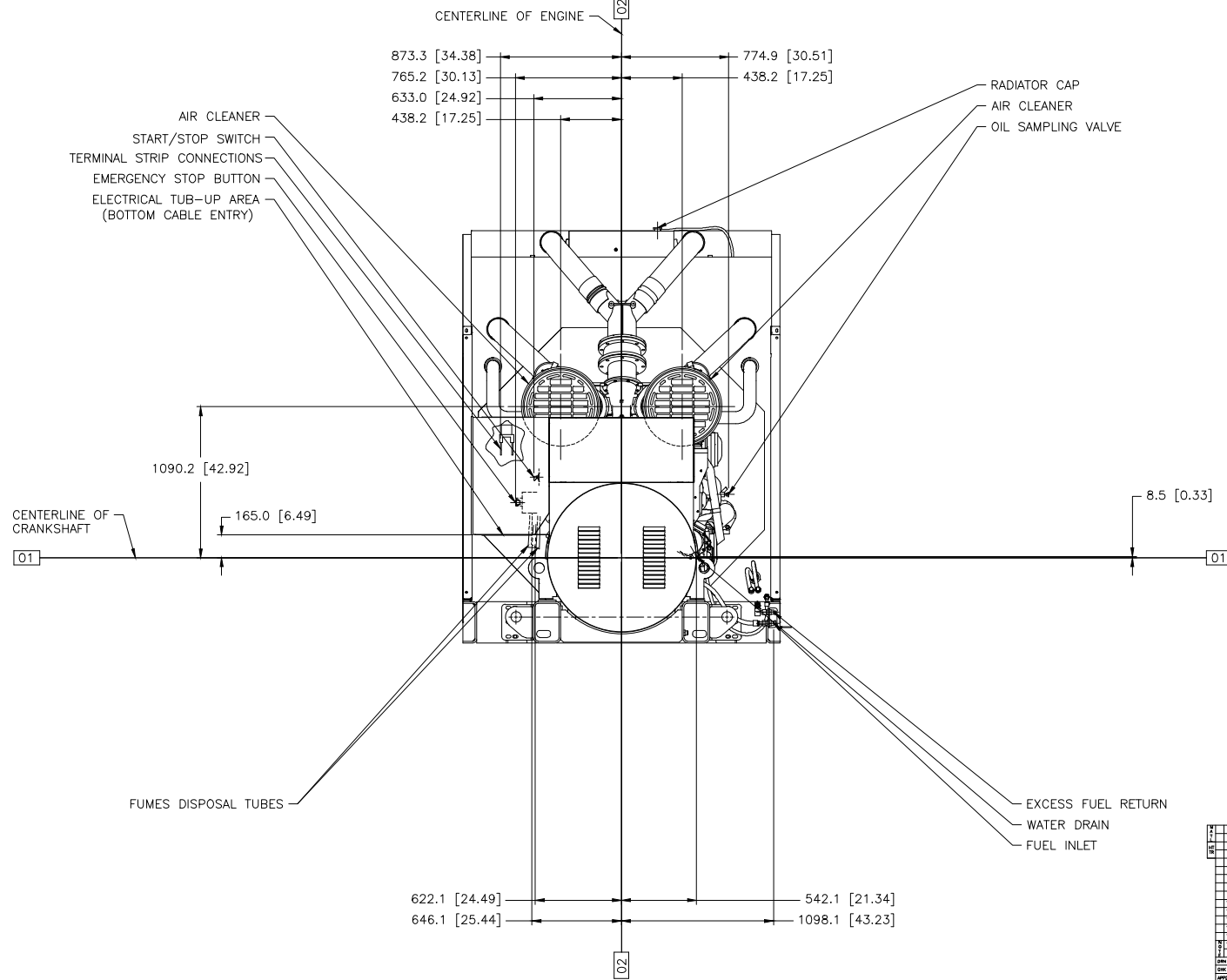
CAT 3516CHD 60HZ HV 2250/2500 KW DWG# 593-3169 CHG 01 METRIC [INCH] REAR VIEW LF-4465 CHG 00 W/ATTACHMENTS SHOWN
