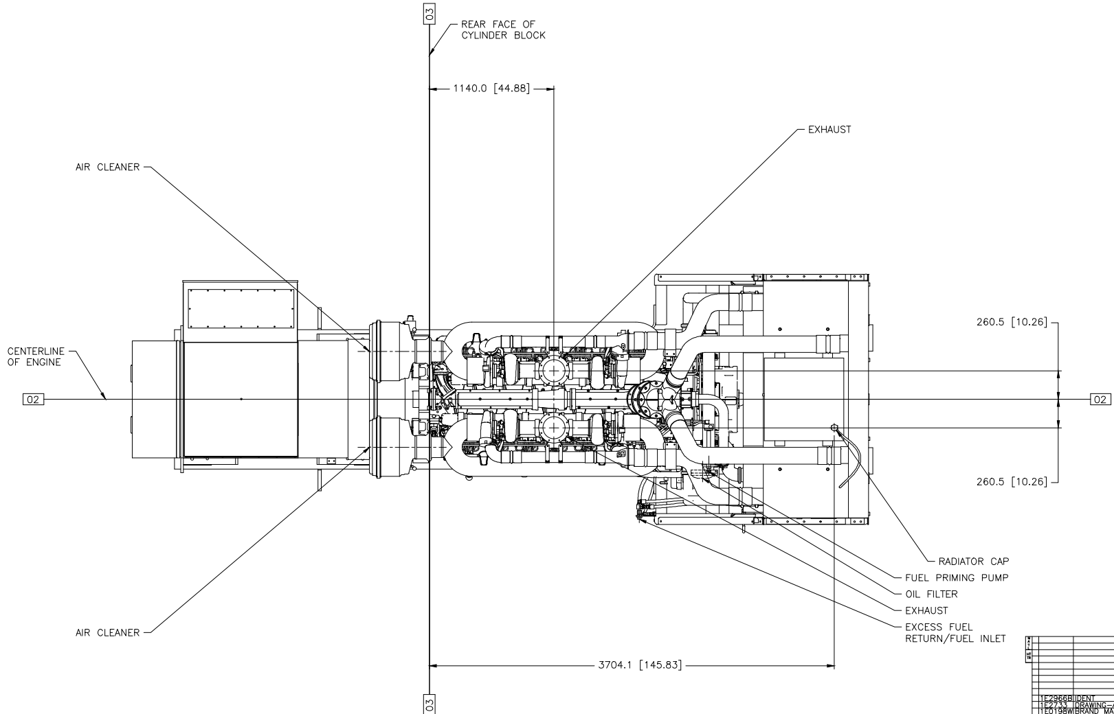
CAT 3516CHD 60HZ HV 2250/2500 KW DWG# 593-3169 CHG 01 METRIC [INCH] TOP VIEW LF-4465 CHG 00 W/ATTACHMENTS SHOWN
