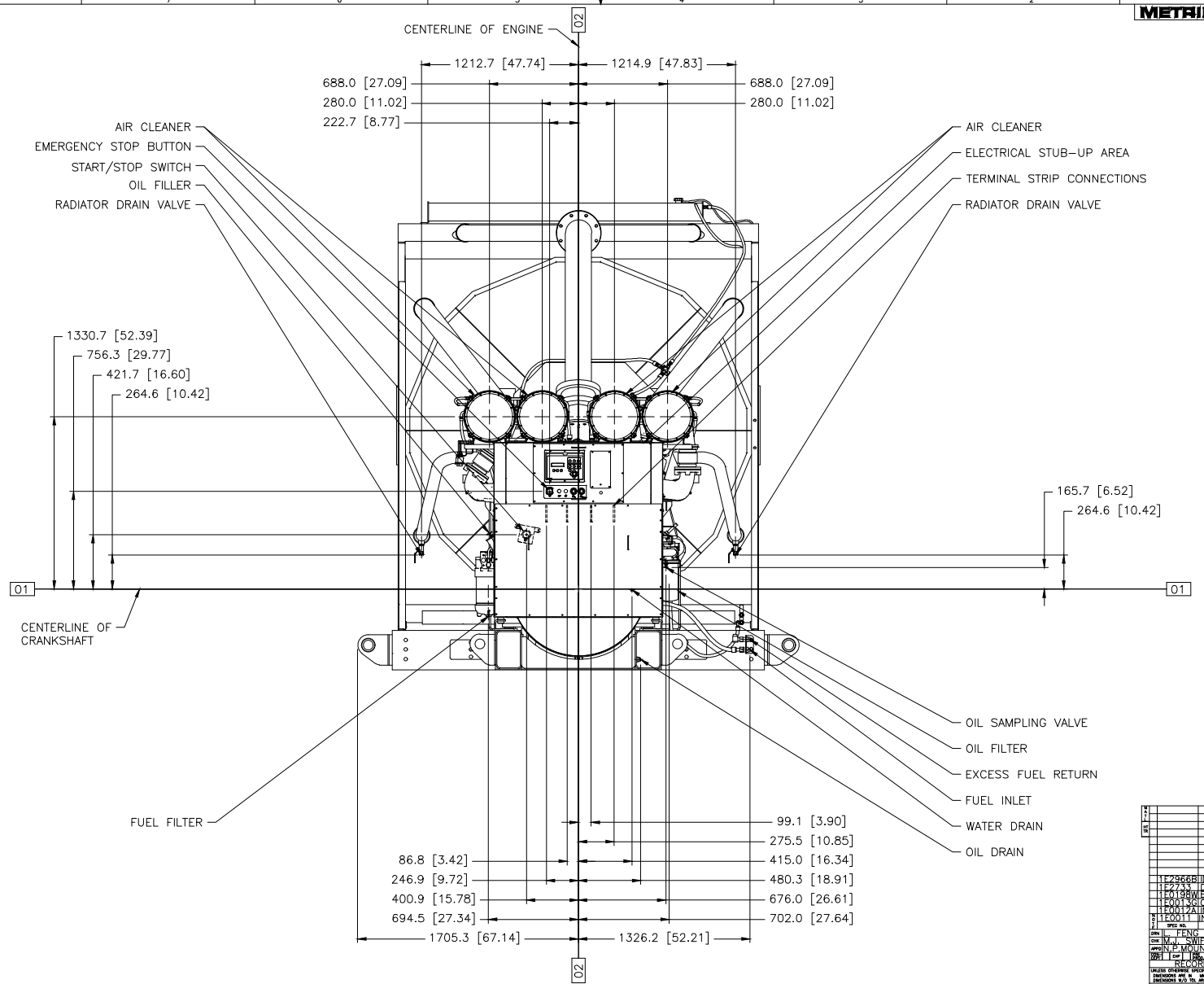
CAT 3516E 60HZ LV/MV PKG 3000KVA DWG# 596-6810 CHG 00 METRIC [INCH] REAR VIEW LF-4610 CHG 00 W/ATTACHMENTS SHOWN
