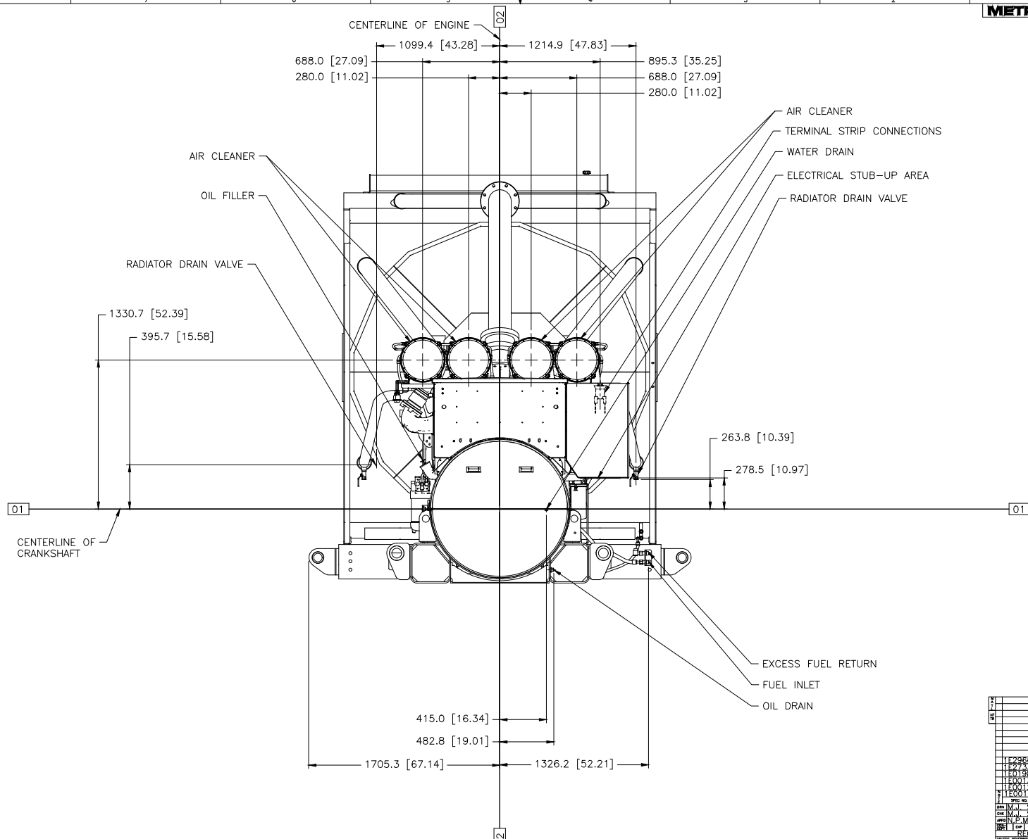
CAT 3516E 60HZ HV PKG 3000KVA DWG# 596-6813 CHG 00 METRIC [INCH] REAR VIEW LF-4609 CHG 00 W/ATTACHMENTS SHOWN
