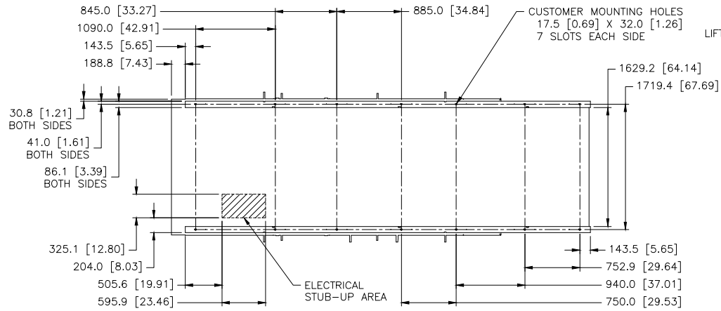
FOOTPRINT (DIMENSIONED OUTLINE VIEW FROM ABOVE)
