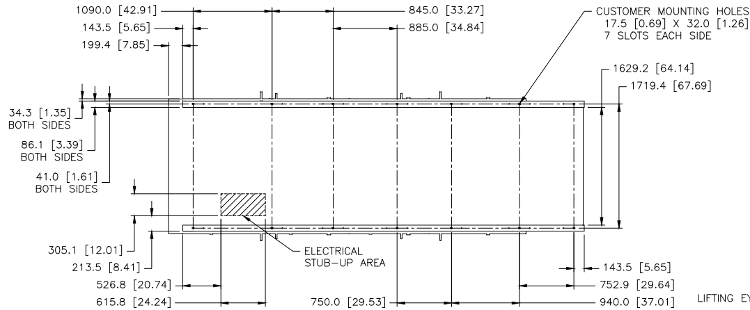
FOOTPRINT (DIMENSIONED OUTLINE VIEW FROM ABOVE)
