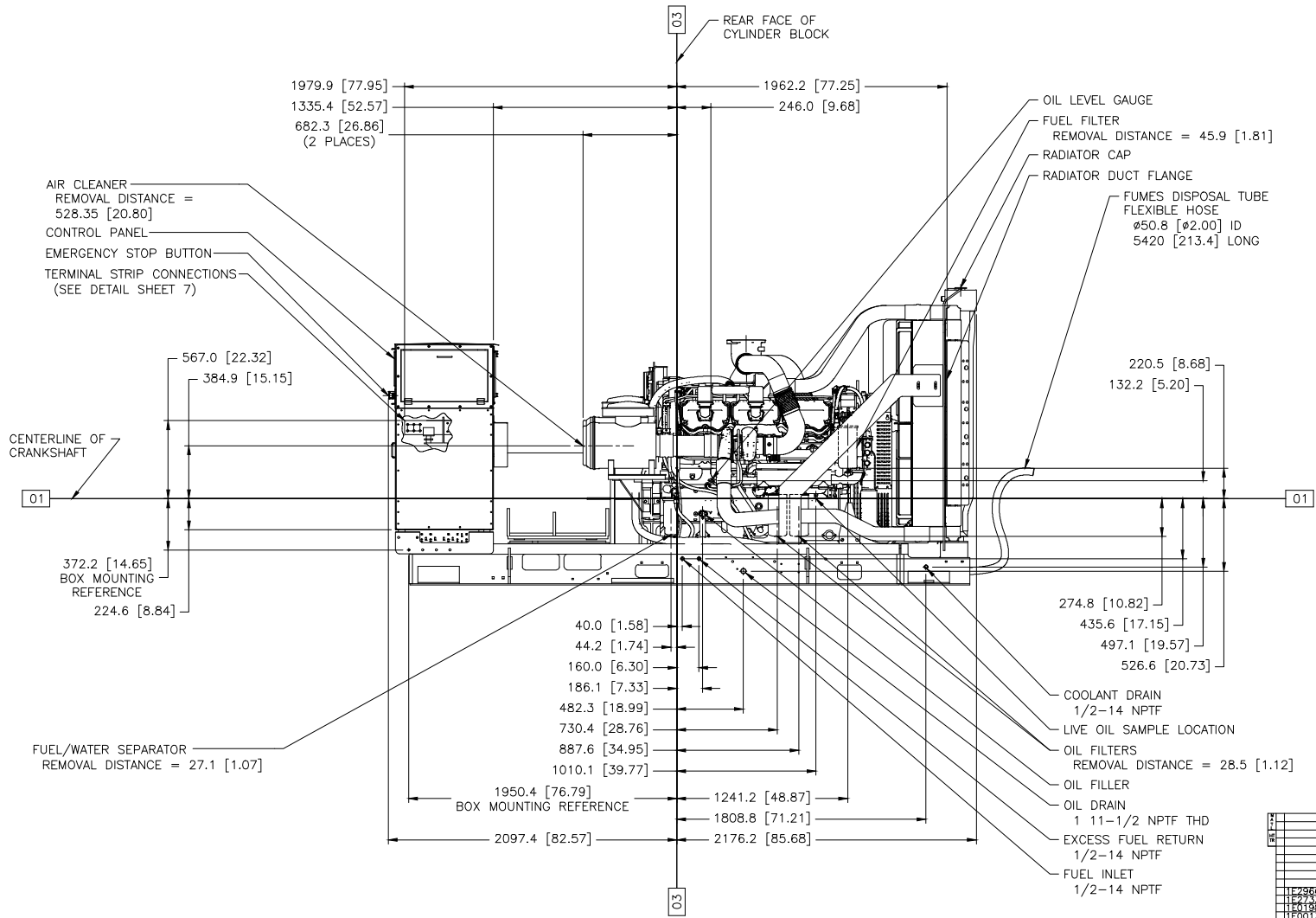
C27 LV 60HZ 1800RPM T2/LOW BSFC DWG# 533-1403 CHG 02 METRIC [INCH] RIGHT SIDE VIEW LF-3344 CHG 06 W/ MANDATORY ATTACHMENTS SHOWN
