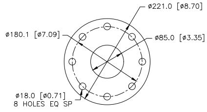
DETAIL OF FUEL INLET SCALE 1=2
