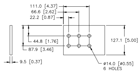
DETAIL OF 311-7115 CHG 01 TERMINAL STRIP CONNECTIONS SCALE 1=2
