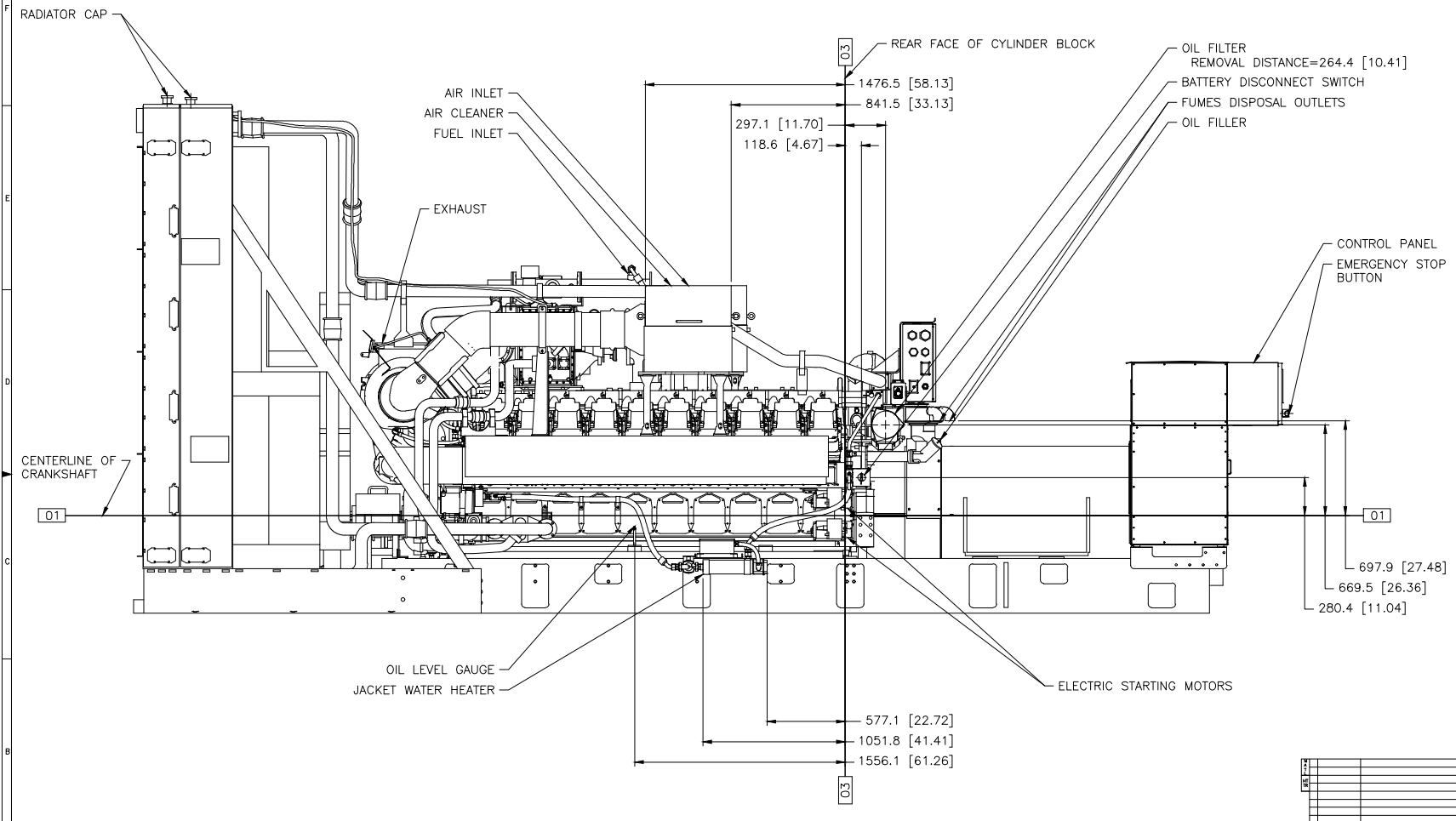
G3520 60HZ 186X GENSET W/ RADIATOR DWG# 579-6101 CHG 01 METRIC [INCH] LEFT SIDE VIEW LF-4381 CHG 03 W/ ATTACHMENTS SHOWN
