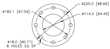
DETAIL OF FUEL INLET SCALE 1=2
