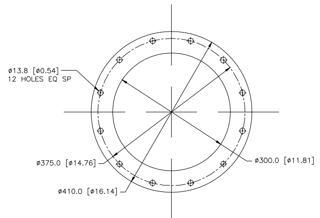
DETAIL OF EXHAUST SCALE 1=2
