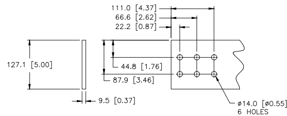
DETAIL OF 311-7115 CHG 01 TERMINAL STRIP CONNECTIONS SCALE 1=2
