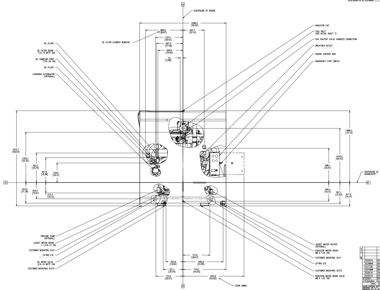
G3512 TA STATIONARY CERT GSE 1800 RPM METRIC [INCH] FRONT VIEW CP-2325 CHG 04 SHOWN W / ATTACHMENTS
