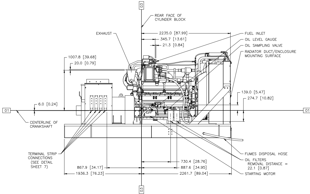
G3412 60HZ WIDE BASE W/ RADIATOR DWG# 601-9225 CHG 00 METRIC [INCH] RIGHT SIDE VIEW LF-4359 CHG 02 W/ ATTACHMENTS SHOWN
