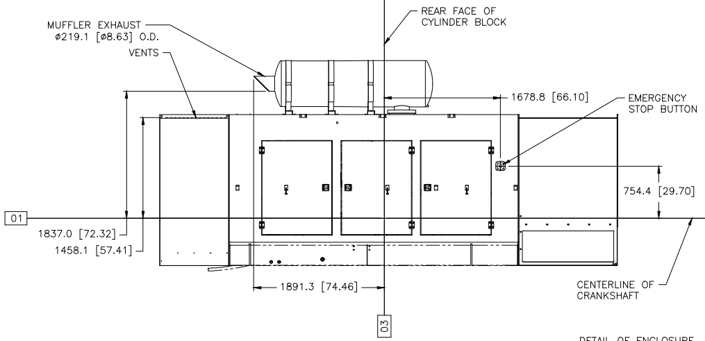
DETAIL OF ENCLOSURE LF-4364 CHG 01
