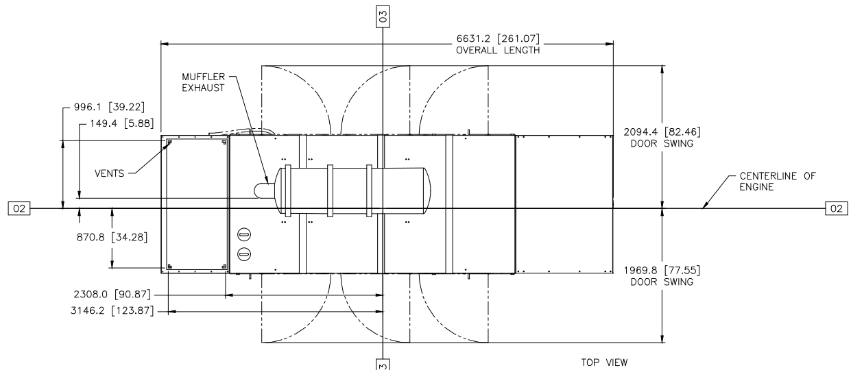
TOP VIEW
